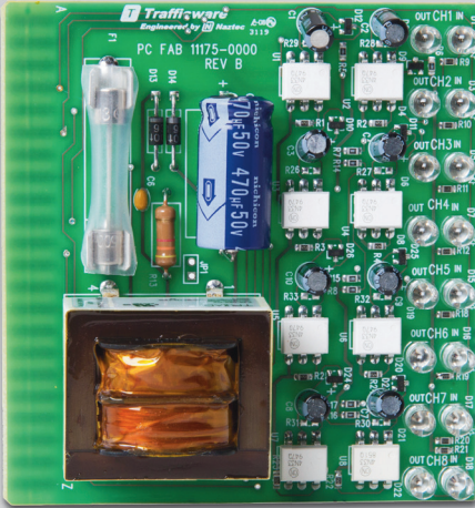
Pictured above: 8-Channel Pedestrian Input Isolator
