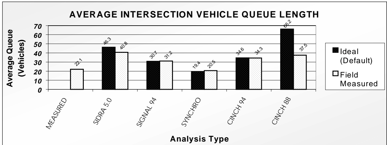
Figure 26 - Average Vehicle Queue Length
