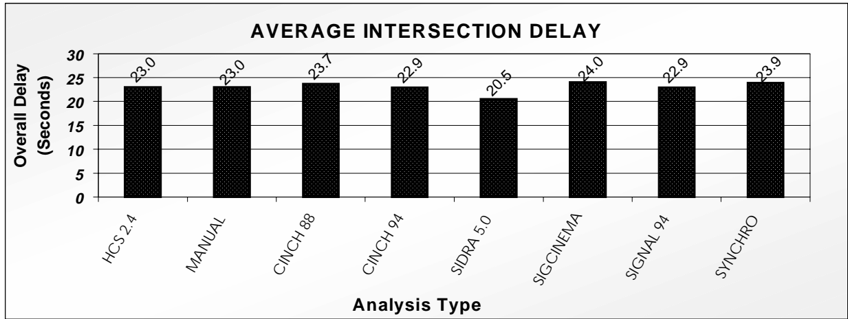
Figure 5 - Average Stopped Delay
