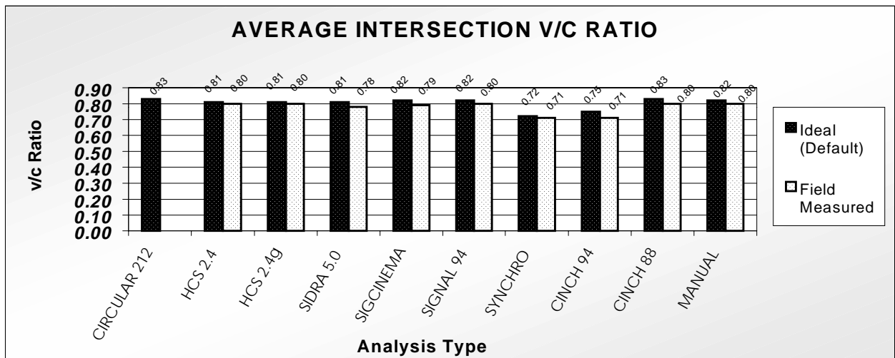
Figure 13 - Volume-to-Capacity Ratio
