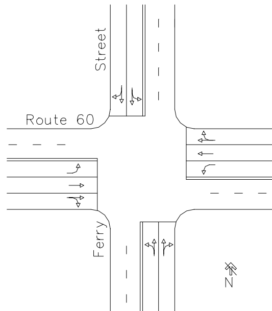
Figure 8 - Intersection B - Route 60 and Ferry Street
