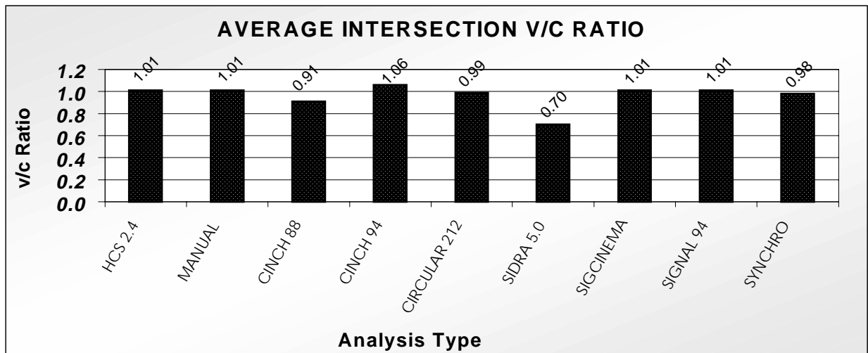
Figure 6 - Volume-to-Capacity Ratio
