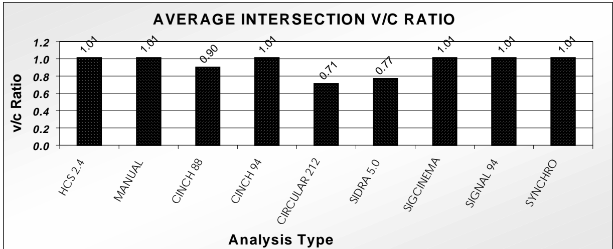
Figure 2 - Volume-to-Capacity Ratio
