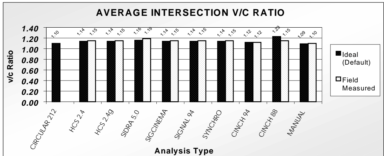
Figure 25 - Volume-to-Capacity Ratio
