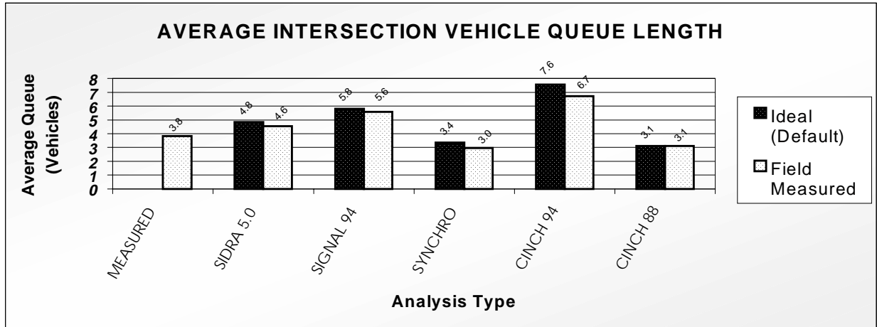
Figure 17 - Average Vehicle Queue Lengths
